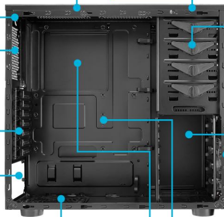
I/O module on the top of bezel-Users can more easily access to USB or AUDIO port.
