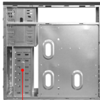
3.5" Drive Bays x 7 External x 2 / Internal x 5
